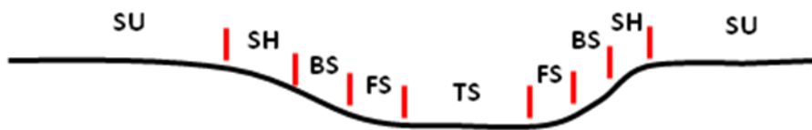
Figure 3. Landscape positions – closed depression example.
